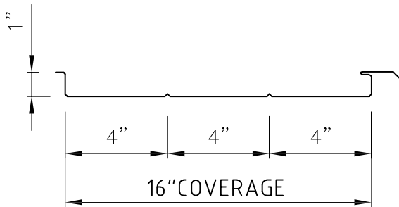
Soffit Profile (Double Pencil Rib Optional)
