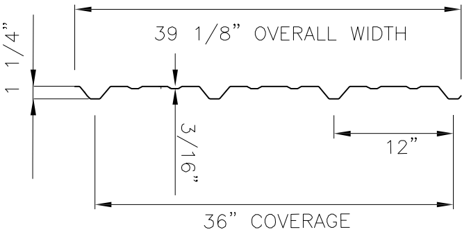
R-PANEL PROFILE (Purlin Bearing Leg)
