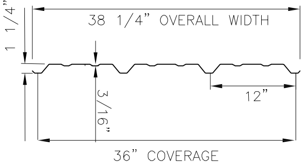
R-PANEL PROFILE - WALLS (Non-Purlin Bearing Leg)
