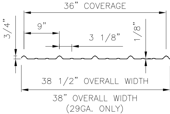
Tuff-Rib PANEL PROFILE
