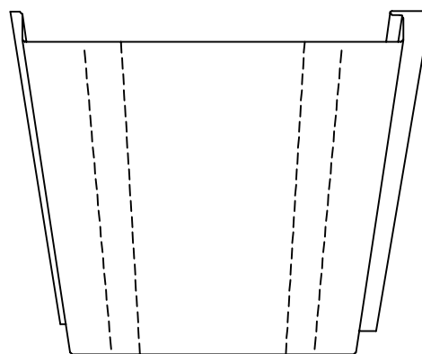
VENTED PANEL
