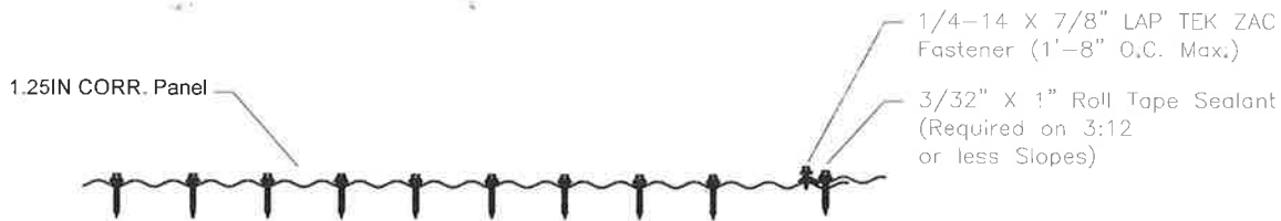
FASTENER PATTERN (@ Eaves, Ridges & Endlaps)
