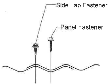
1.25" CORRUGATED PANEL SEAM
